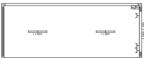
ARS C3L 08 - (LxB) 6,058m x 2,438m; RH = 2,50m
